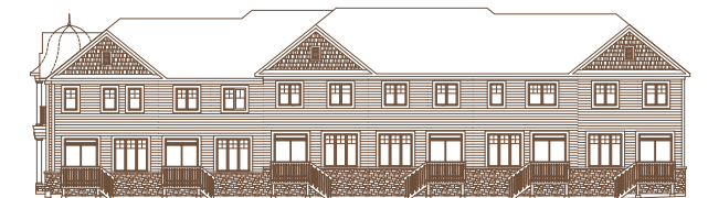
Rear Elevation A (Building 6)
