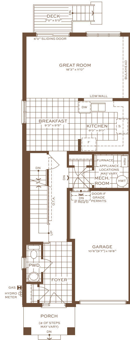
Main Floor Elevation A
