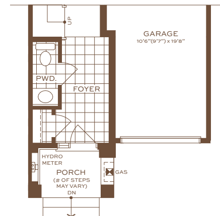
Partial Main Floor Elevation A MOD.
