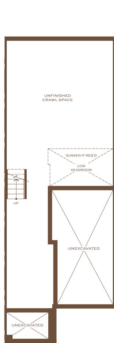
Crawl Space Elevation A/A MOD./B/B MOD.
