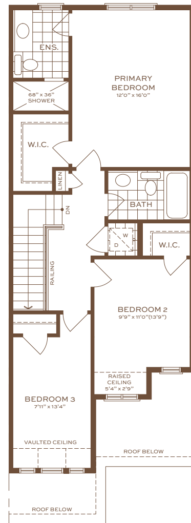
Second Floor Elevation A
