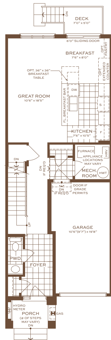
Main Floor Elevation A
