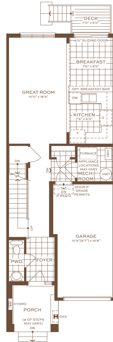
Main Floor Elevation A/A MOD./B
