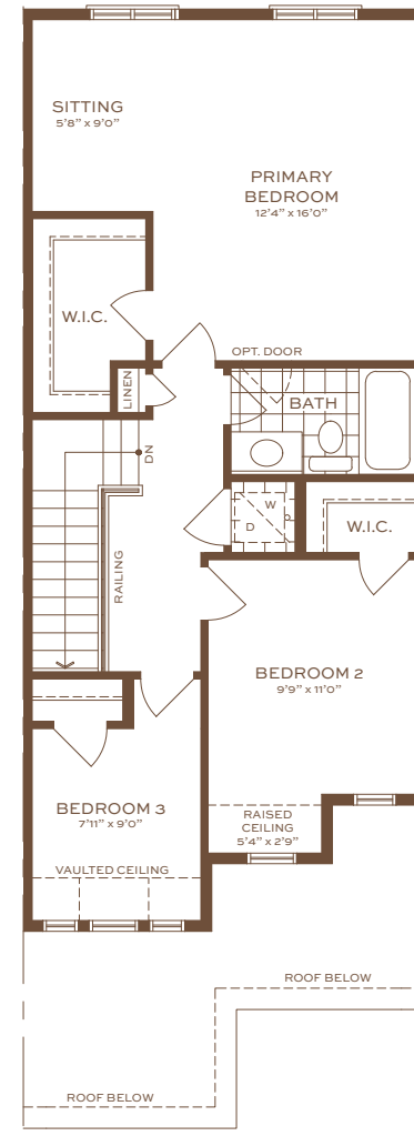
Second Floor Elevation A/A MOD.
